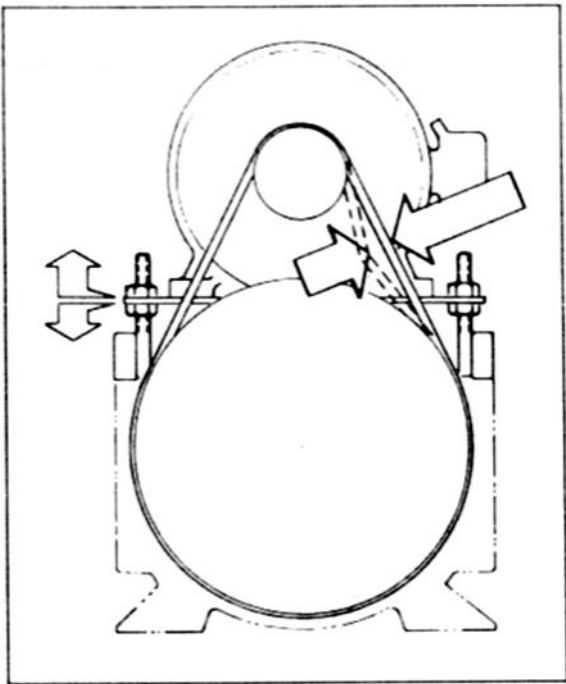
BELT DEFLECTION SHOWN
